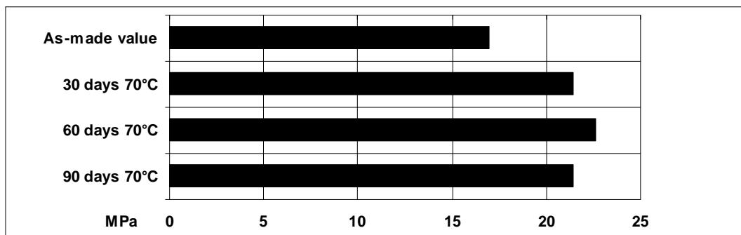
Lap shear strength versus heat ageing
